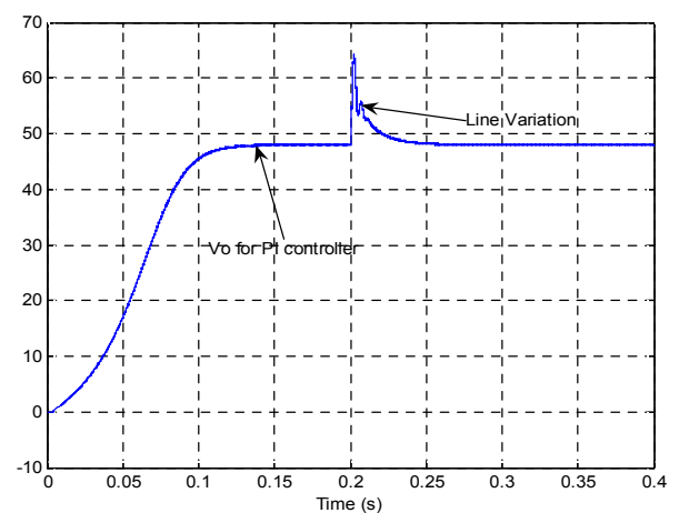
Fig. 11. Response of the average output voltage of the SEPIC converter using the PI controller for the step change in V_{in} (from 12V - 15V at t=0.2s ).
