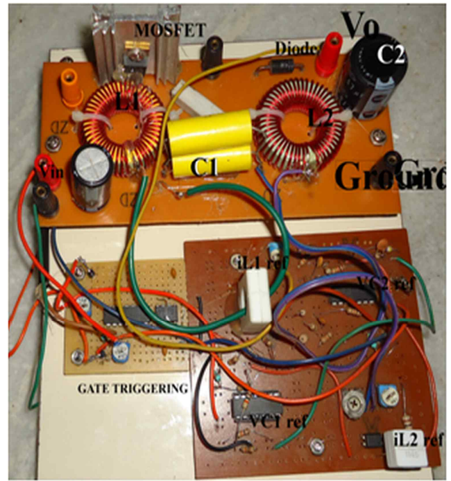
Fig. 29. Photograph of Designed Laboratory type SMC controlled SEPIC.
