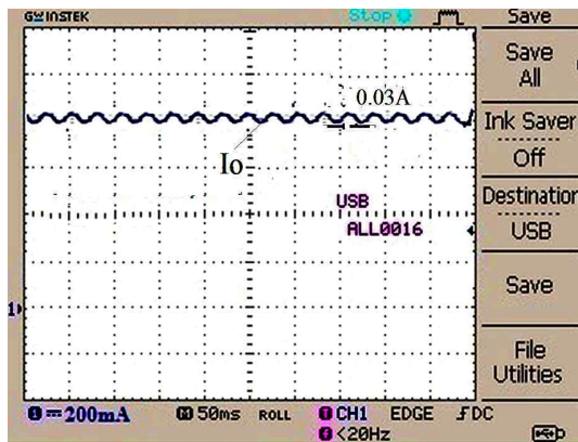
Fig. 24. Response of the SEPIC using the SMC for load current steady state condition for load R = 60Ω, v_{in}=12V .
