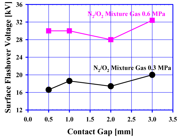
Fig. 3. Surface flashover voltage with the gap of poor contact in N_2/O_2 Mixture gas(8/2)
