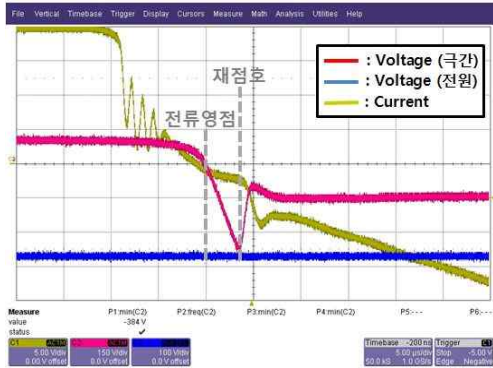
Fig. 8. Waveform of experiment
