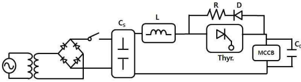
Fig. 5. Measurement circuit
