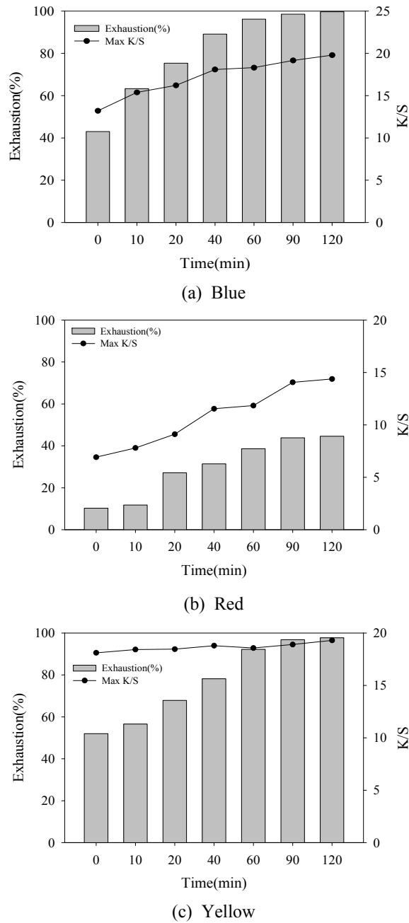
Figure 7. Exhaustion and K/S values depending on dyeing time.
