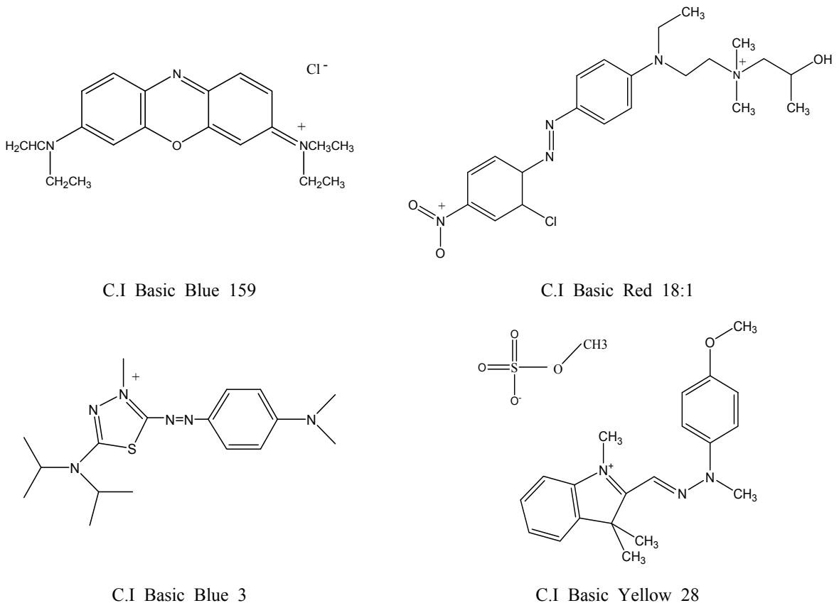
Figure 2. Cationic dyes used for this study.
