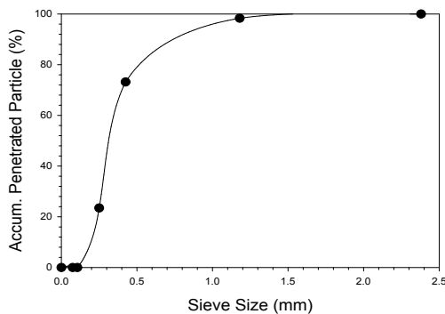
Fig. 1. Particulate distribution of contaminated soil used in this soil by sieving.
