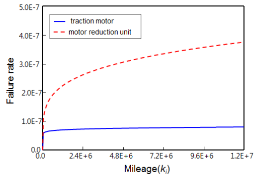
Fig. 7. Failure rate curves of MRU and TM
