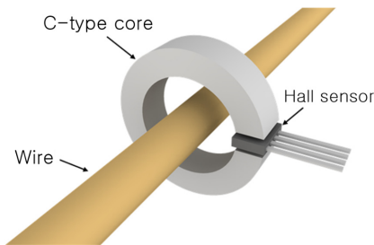
Fig. 1. Structure of a open-loop current sensor
