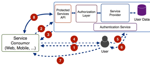
Fig. 2. Standard OAuth roles and operation flow
