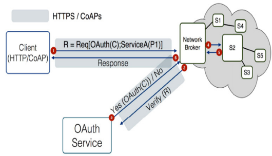
Fig. 3. Network Broker Communication
