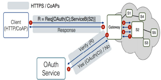
Fig. 4. Gateway-Based Communication
