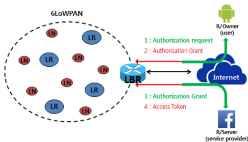
Fig. 7. The proposed Authentication Framework
