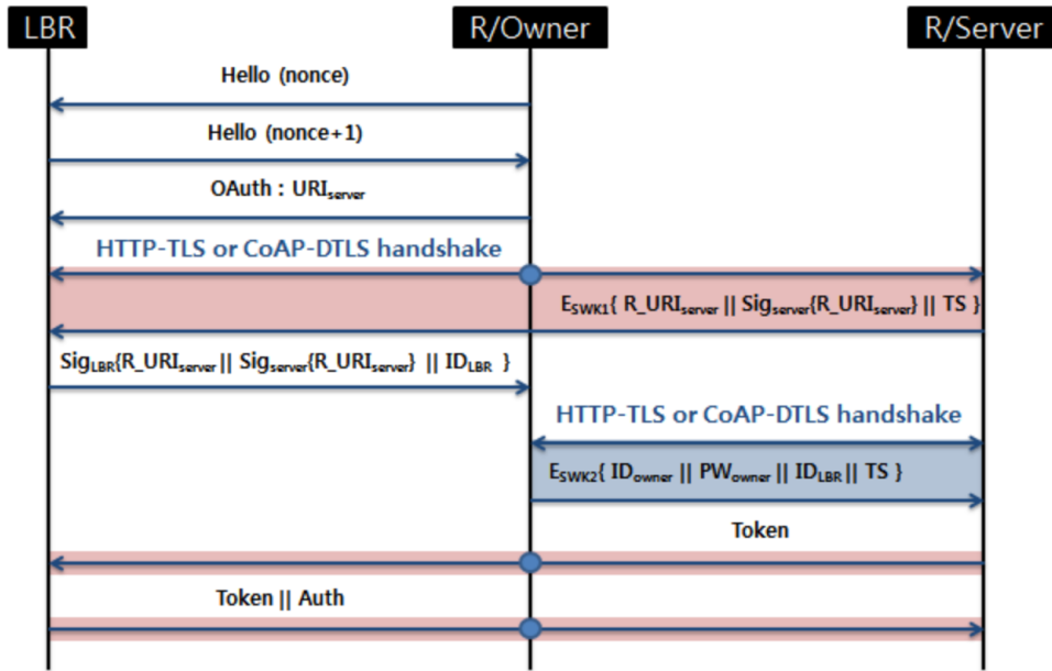
Fig. 8. The proposed User Authentication procedure
