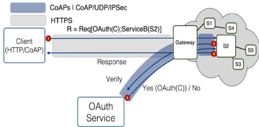
Fig. 6. Hybrid Gateway-Based Communication
