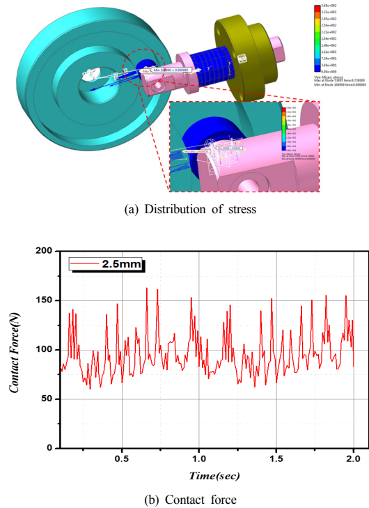
Fig. 5. Result of dynamic analysis case of d=2.5mm
