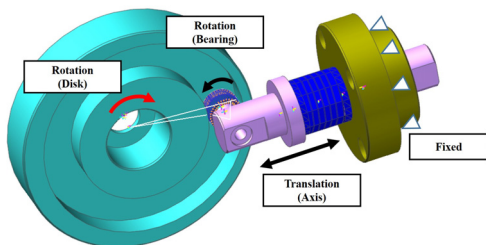
Fig. 4. Dynamic model of the oscillation module
