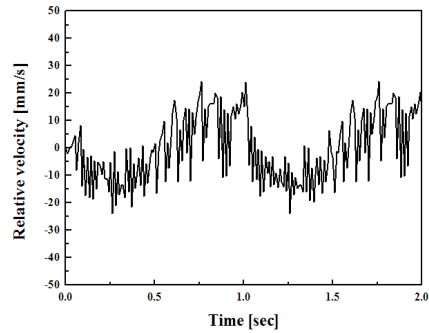
Fig. 10. Result of relative velocity case of d=1.5mm
