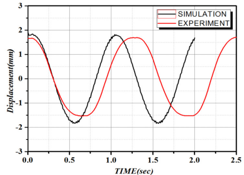
Fig. 12. Displacement of the oscillation module according to time
