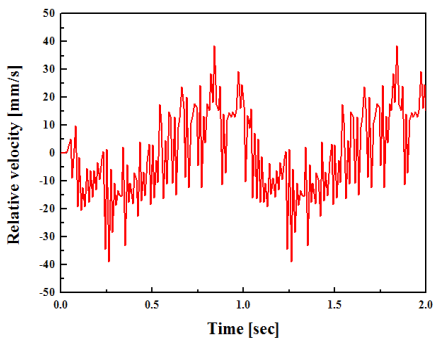
Fig. 9. Result of relative velocity case of d=2.0mm
