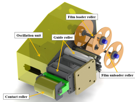
Fig. 1. The structure of abrasive film polishing system
