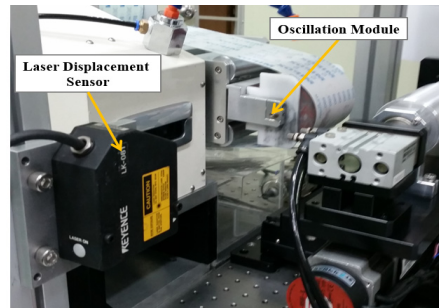
Fig. 11. Photograph of experiment set-up for measurement of displacement
