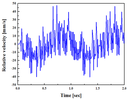
Fig. 8. Result of relative velocity case of d=2.5mm
