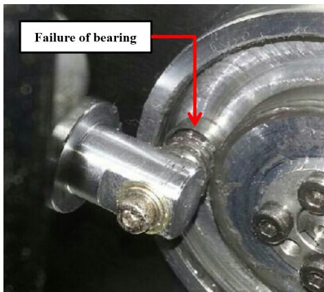
Fig. 3. Failure of bearing in the oscillation module
