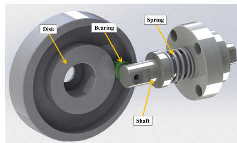
Fig. 2. The structure of the oscillation module
