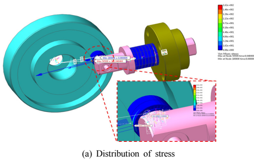
Fig. 5. Result of dynamic analysis case of d=2.5mm
