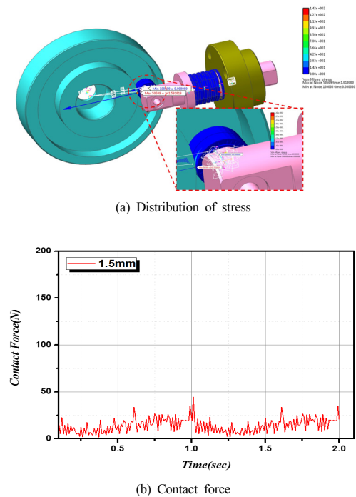
Fig. 7. Result of dynamic analysis case of d=1.5mm
