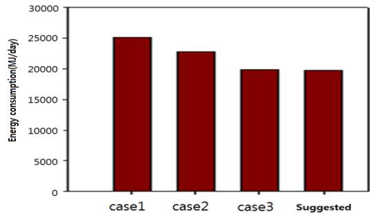
Fig. 10. Energy consumptions with Cases. (lowest/highest temperatures in a day: 19℃ /29.6℃)
