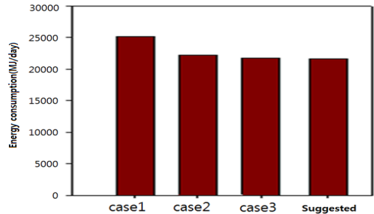
Fig. 9. Energy consumptions with Cases. (lowest/highest temperatures in a day: 17℃/29.5℃)
