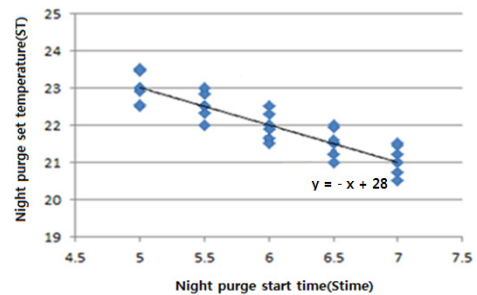
Fig. 8. Set temperatures for night-purge control system with start time changes.
