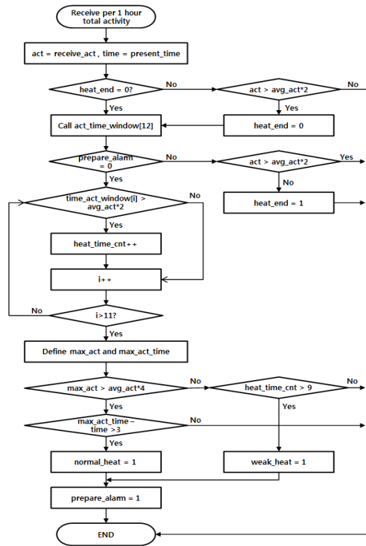
Fig. 8. Estrus detection algorithm using activities
