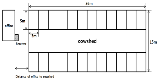
(a) Construct of cowshed used in experiments
