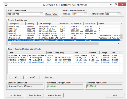
Fig. 4. Battery life simulation3
