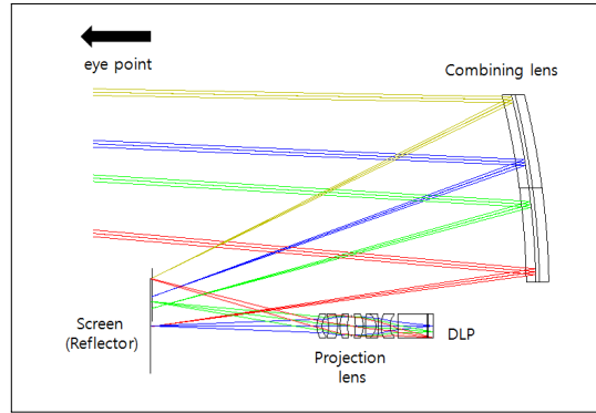
Fig. 7. Layout of The HUD Optical System
