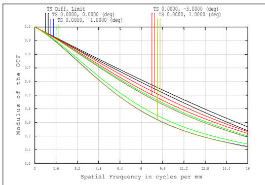
Fig. 13. MTF of The Combiner(edge)
