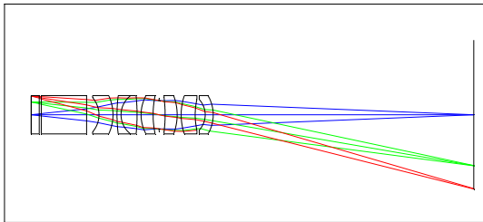
Fig. 9. Layout of The Projection Lens
