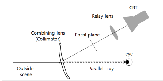
Fig. 2. Typical Reflective Optical System of a HUD
