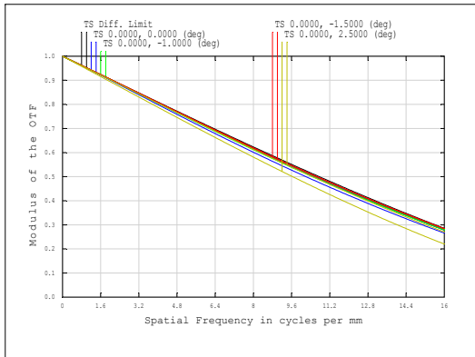
Fig. 12. MTF of The Combiner(Center)
