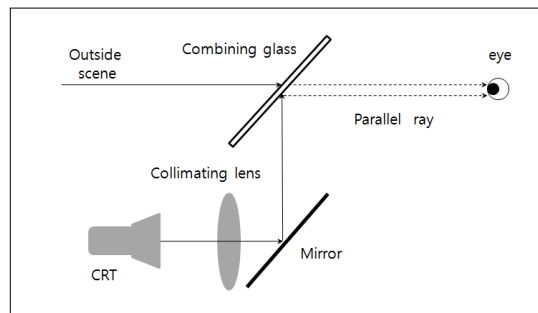
Fig. 1. Typical Refractive Optical System of a HUD
