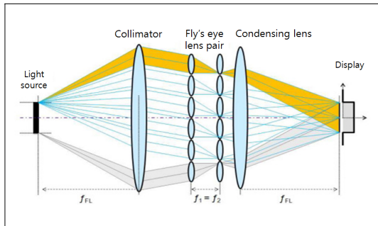
Fig. 4. Beam Homogenizer with Fly's eye lens
