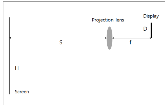
Fig. 8. Schematic of a Projection Optics
