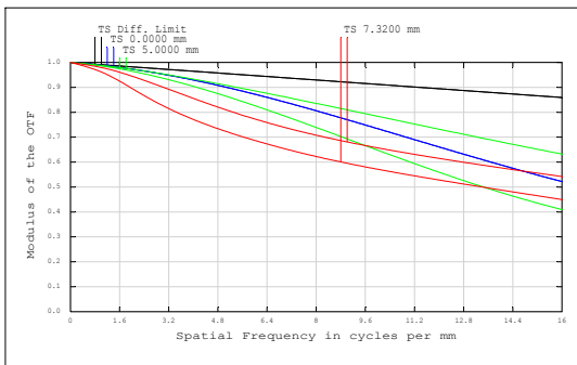
Fig. 10. MTF of The Projection Lens
