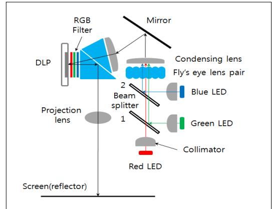
Fig. 5. DLP Projector's Optics with Fly's eye lens
