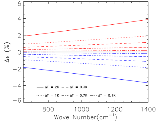
Fig. 4. The emissivity error resulting from incorrect temperatures of the sample. Spectral errors are presented as percent change in emissivity from the correct emissivity value.
