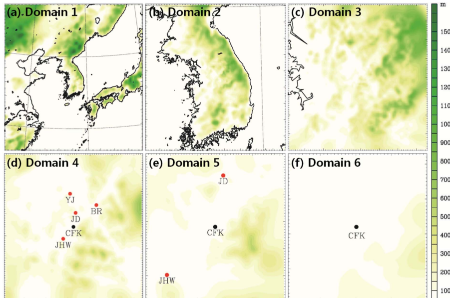
Fig. 3. Model domains and topography (unit: meters).
