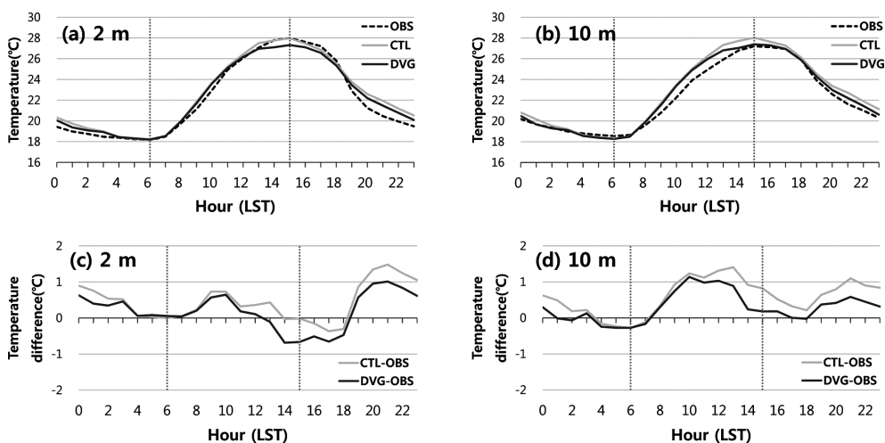
Fig. 10. Hourly mean diurnal cycle of (a) simulated 2 m and observed 2 m air temperatures (°C) and (c) difference between observed 2 m and simulated 2 m temperatures at CFK in domain 4. (b) and (d) same as (a) and (c), but for simulated 10 m and observed 9 m air temperature (i.e., averages of the observed 1 m and 3 m air temperatures).
