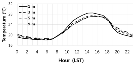
Fig. 9. Same as Fig. 7, but for observed air temperatures (°C) at 1 m, 3 m, 5 m, and 9 m.
