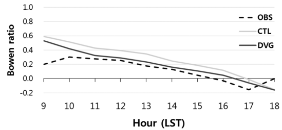
Fig. 8. Same as Fig. 7, but for Bowen ratio.
