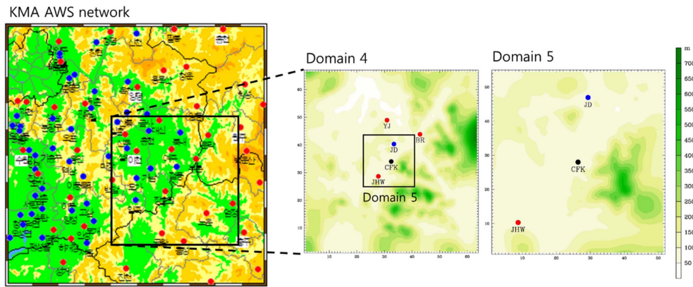
Fig. 2. The national observation sites around the CFK site. Model precipitation is compared with the observed precipitation at Janghowon (JHW), Jeomdong (JD), Yeoju (YJ), and Buron (BR). Model topography is shaded in green.
