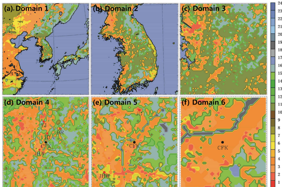
Fig. 4. Same as Fig. 3, but for model land-cover type. Also see Table 1 for land-cover category information.
