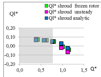
Figure 11. Fluid leakages at impeller/diffuser shroud
