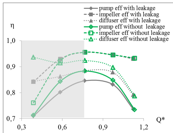
Figure 8. Impeller and pump efficiency \eta
