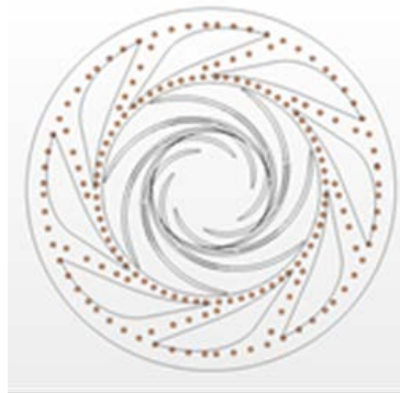
Fig. 4. Probes for frozen rotor calculations.
