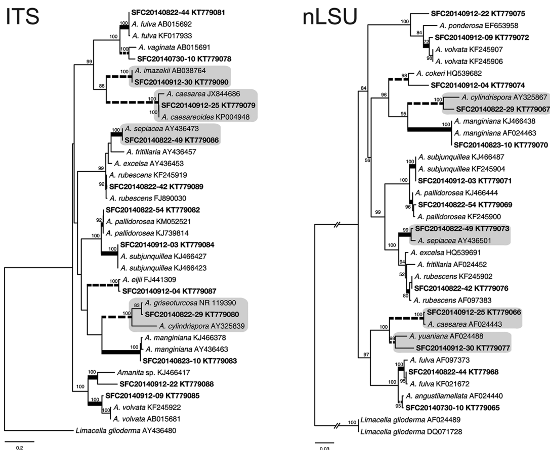
Fig. 1. Phylogenetic trees for Amanita species based on maximum likelihood analysis of internal transcribed spacer (ITS) and large subunit of nuclear ribosomal RNA (nLSU) sequences. Bootstrap scores of > 50 are presented at the nodes. The scale bar indicates the number of nucleotide substitutions per site. Thickened branches on the root nodes represent identical results between ITS and nLSU, while dotted lines represent the branches which have incongruent results between the ITS and nLSU. Gray boxes indicate the new species found in Korea.
