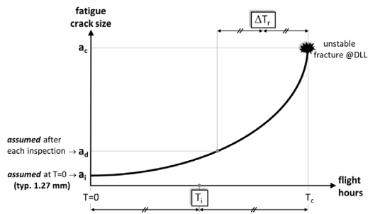
Fig. 1 Determination of initial inspection time T_i and recurring inspection interval \Delta T_r in the slow crack growth damage tolerance concept
