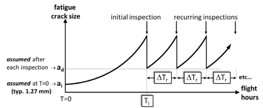
Fig. 2 In-service inspections for fatigue cracks. After each inspection the size of the assumed crack is reset to its in-service detectable size
