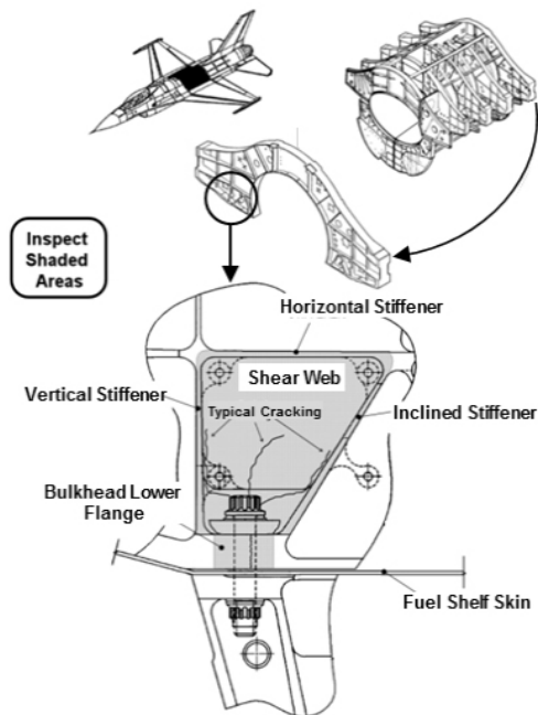
Fig. 4 Easy visual inspection for large cracks in flanges and web of the upper FS 341 bulkhead [10]
