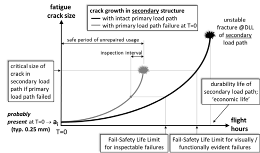
Fig. 5 Determination of the fail-safety life limit from the crack growth curve for adjacent structure [9]. The visual inspection interval usually is aligned with phased maintenance. The initial inspection is not prescribed in ref. [9], but is usually taken as half the safe period of unrepaired usage
