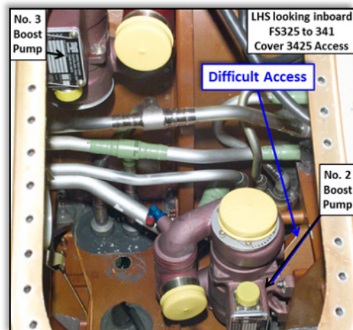
Fig. 3 Difficult access to the fracture critical F-16 fuel shelf joint bolt holes at fuselage station FS 341 [10]
