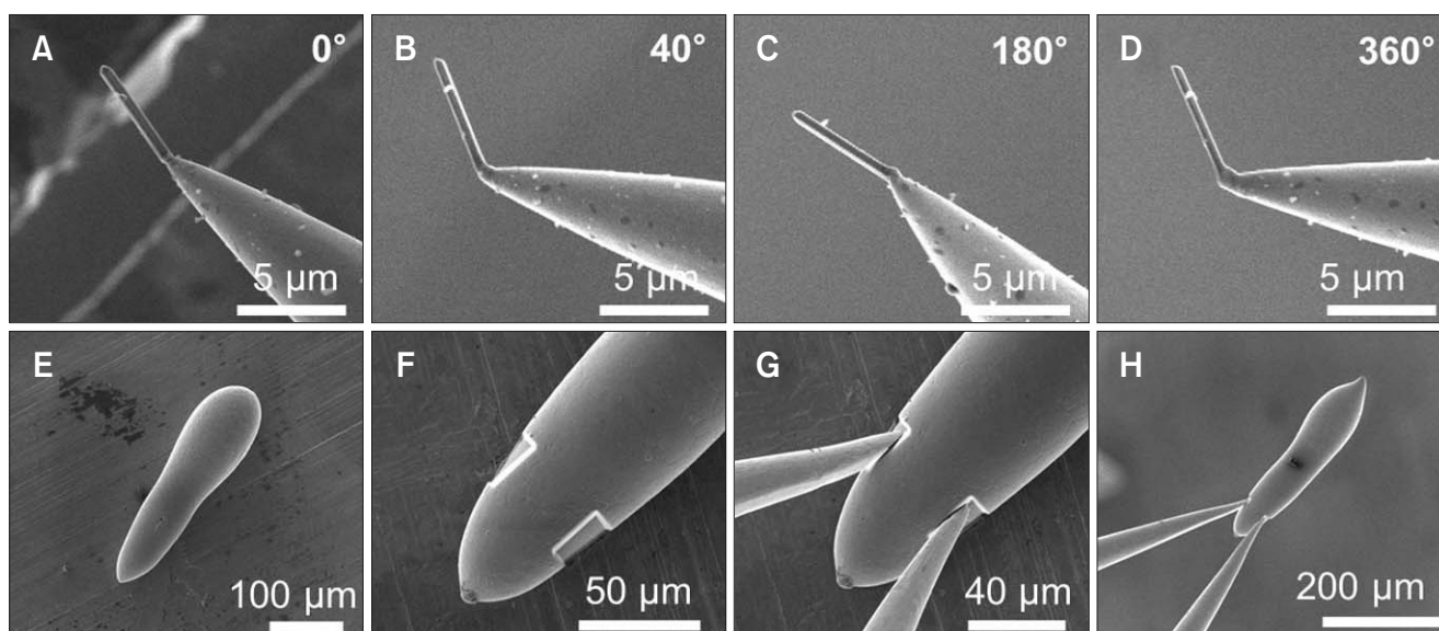
Fig. 5. Applications of the rotation tip and gripper. (A-D) A nanowire picked with any angle, which can be aligned by a rotation tip. (E-H) A lifting-out process by a gripper.
