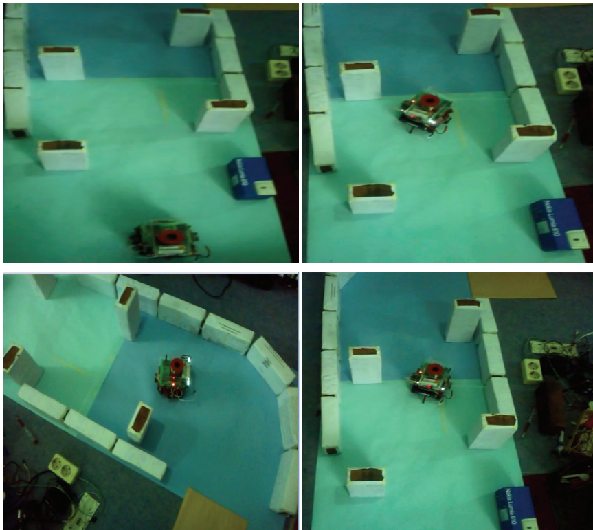
Fig. 6. Experiment with single robot.
