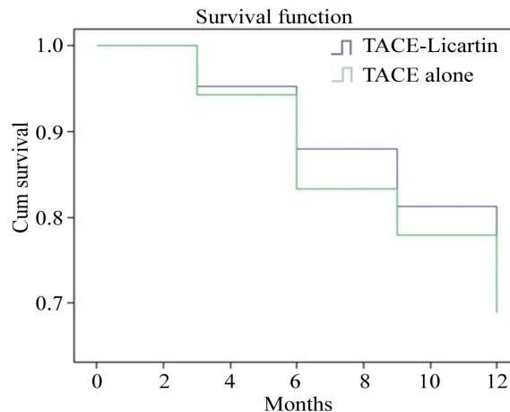
Figure 2. Survival Curve of Life Table Method for Licartin plus TACE versus TACE alone *(P=0.041). *Log-rank test for comparing the statistical difference of survival curve. P<0.05 was considered having significant difference
