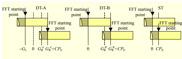
Fig. 6. Three types of time synchronization schemes: DT-A, DT-B, and ST.
