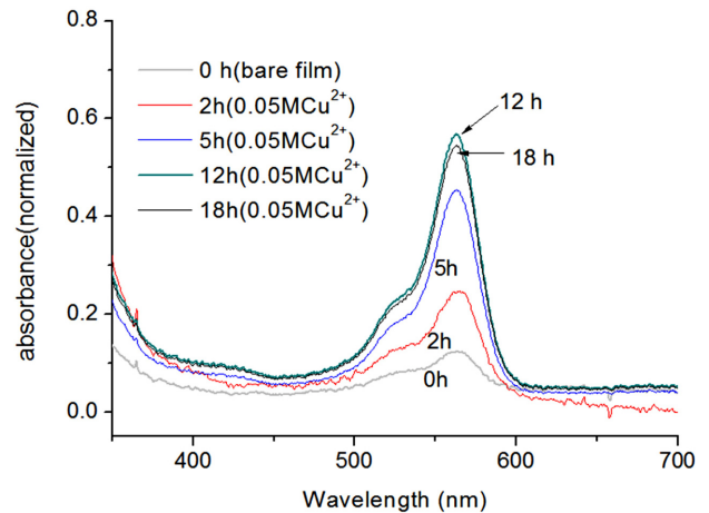
Figure 8. Absorption spectrum of a film (F-Rh1) treated with Cu(II) solution for several hours.
