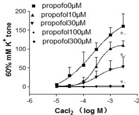
Fig. 5. CaCl 2 -induced contraction in Ca 2+ -free solution containing 60 mmol/L K + in the absence (n=5) and presence of propofol (10 to 300 μmol/L, n=5). A significant difference in E max between control and propofol-treated groups is indicated by an asterisk (p < 0.001).
