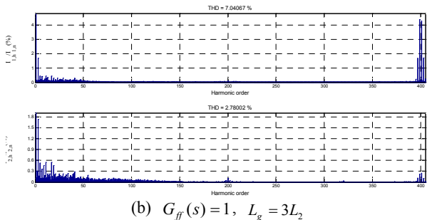
Fig. 9. Simulations under weak and stiff grid conditions.
