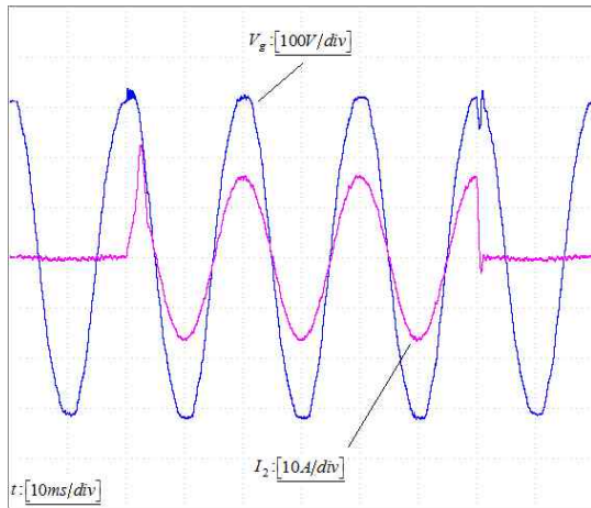
Fig. 10. Experimental waveforms of grid voltage and current in weak grid ( L_g=1\text{mH} ).
