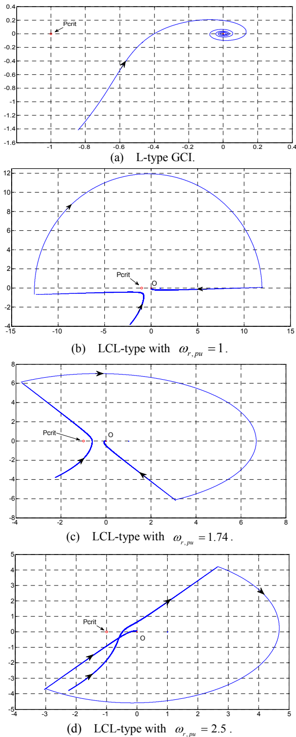
Fig. 2. Open-loop Nyquist diagram of L-type and LCL-type GCI.
