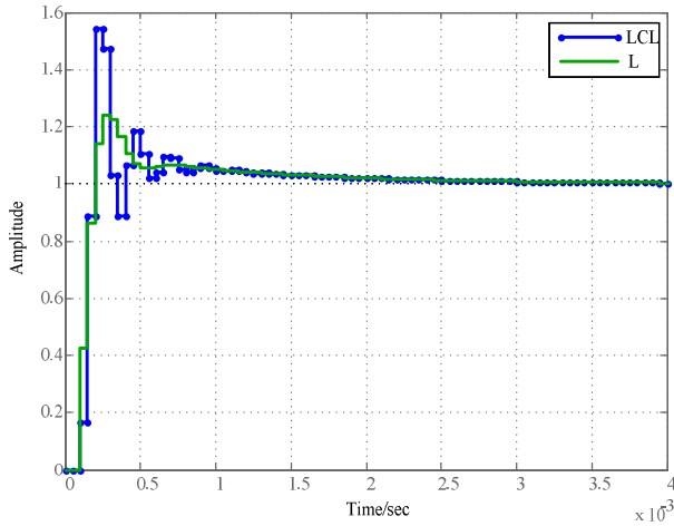
Fig. 4. Step responses of L-GCI and LCL-GCI.
