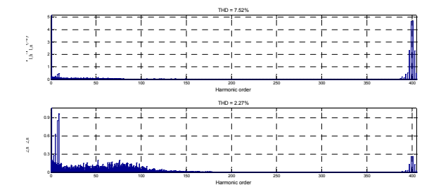
(c) Harmonic spectrum. (Subscripts h and n denote harmonics and fundamental components respectively.) Fig. 7. Simulations under weak and stiff grid conditions.
