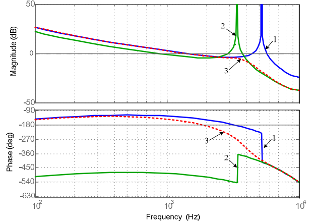
Fig. 6. Open-loop Bode diagram against grid impedance.
