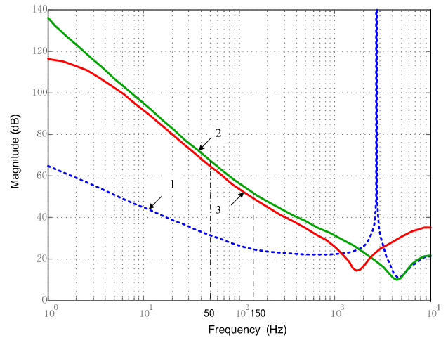
Fig. 5. Output impedance of LCL-GCI.
