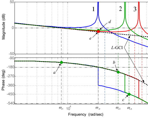
Fig. 3. Open-loop Bode diagram of LCL-type GCI against \omega_{r,pu} with L-type counterpart (dashed line) as the benchmark.
