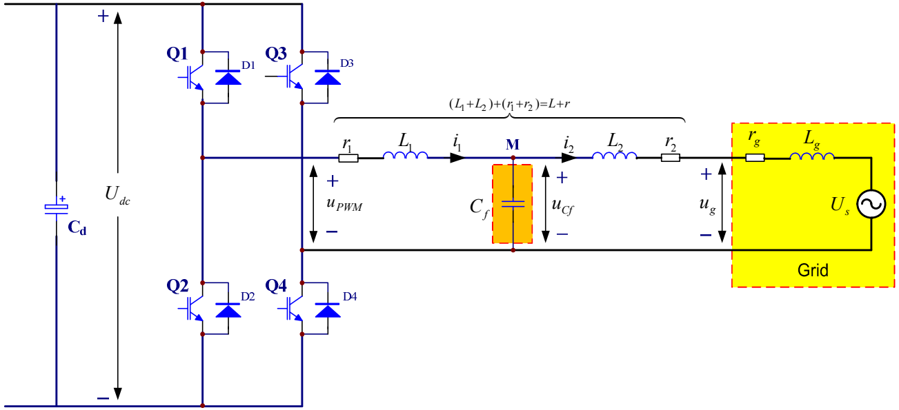
(a) Topology.
