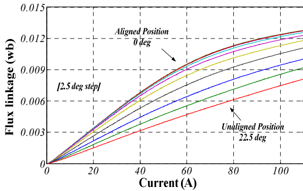
Fig. 13. Measured flux-linkage curves.
