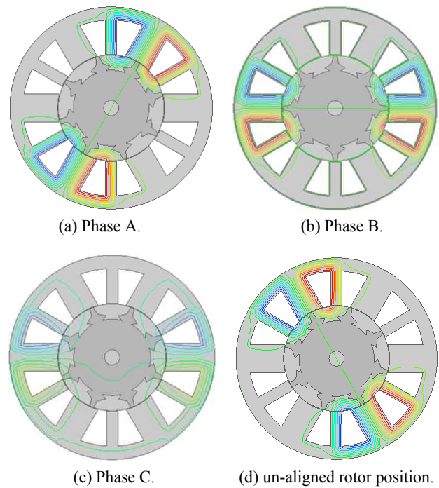
Fig. 5. Magnetic flux distribution.
