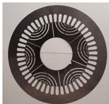
Fig. 13. 6-pole synchronous reluctance machine lamination.
