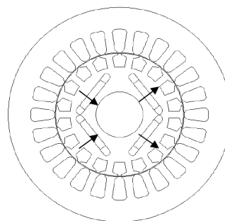
Fig. 12. 2-pole line start PM – rotor has both interior permanent magnets and a cage.
