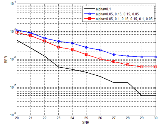
Fig. 8. BER performance when the block length is 4096×5
