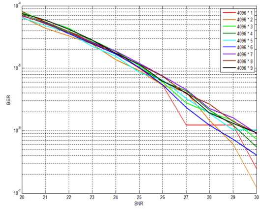
Fig. 4. Performance according to the block length of ITIC
