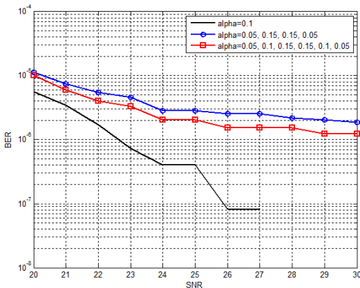
Fig. 7. BER performance when the block length is 4096×3
