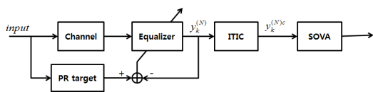
Fig. 2. Block diagram of ITI Cancellation
