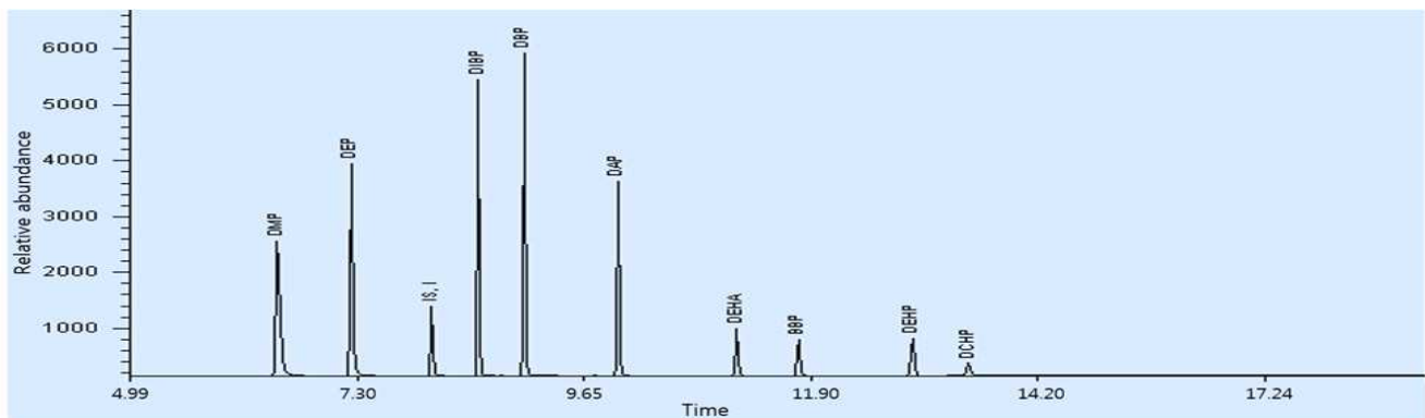
Fig. 1. Total ion chromatogram of nine regulated phthalates and internal standard
