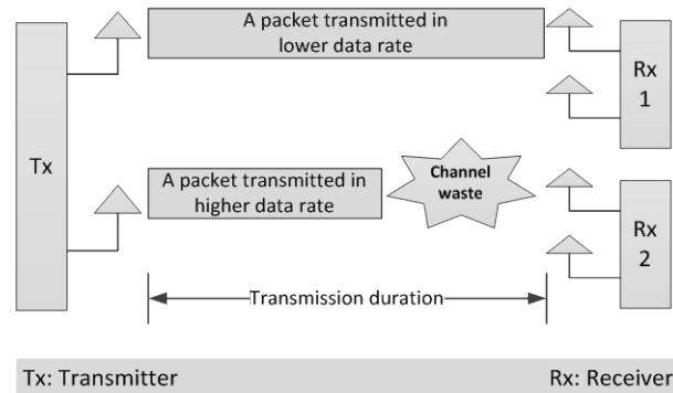
Fig. 1. Capacity loss caused by variable data rates in MU-MIMO
