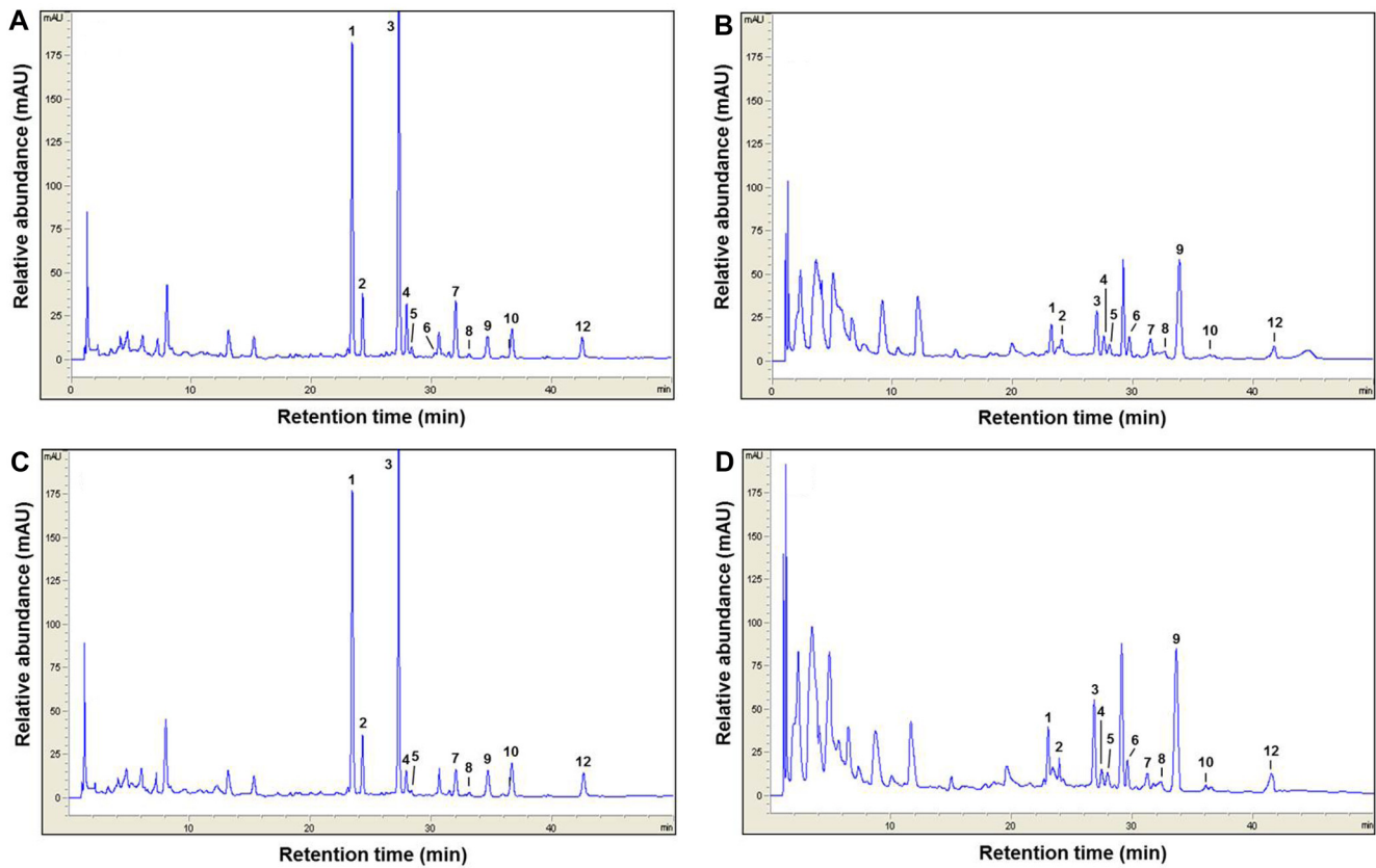
Fig. 3. Profile of HPLC chromatogram from isoflavone extracts.
