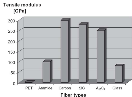
Fig. 2. Fiber types and tensile modulus [7]
