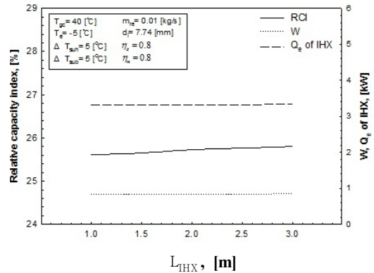
Fig. 5 RCI, W, Qe of IHX with respect to variation of Length of internal heat exchanger
