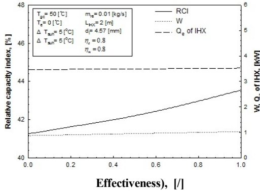
Fig. 6 RCI, W, Qe of IHX with respect to variation of effectiveness of internal heat exchanger
