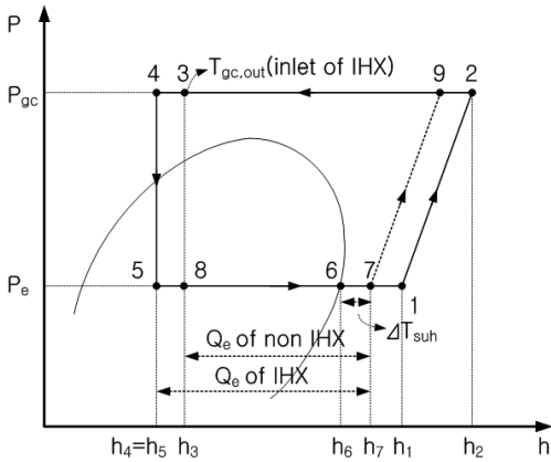
Fig. 2 Vapor compression refrigeration cycle of R-1270 with internal heat exchanger on P-h property plots.
