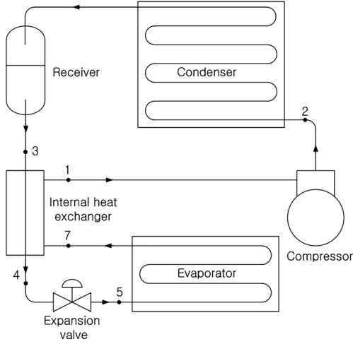
Fig. 1 Schematic diagram of R-1270 refrigeration system with internal heat exchanger.
