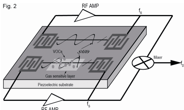
Figure 2. Illustration on how SAW Sensor Works. A second SAW device is used as a reference to minimize the temperature drift ( f_S is sample frequency, f_R is reference frequency and f_D is frequency difference)
