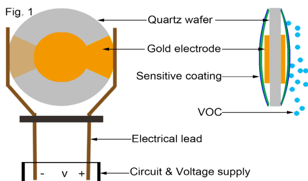
Figure 1. Schematics of a QCM Sensor
