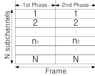
Fig. 2. A frame structure
