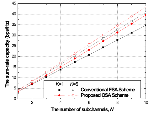
Fig. 4. The sum-rate capacity versus the number of subchannels
