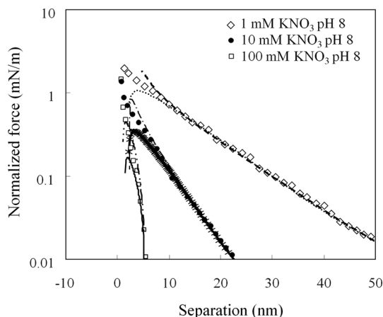
Fig. 5. Approaching force curve as a function of the separation between the zirconium dioxide sphere and the glutathione layer in 1, 10, 100 mM potassium nitrate at pH 8.
