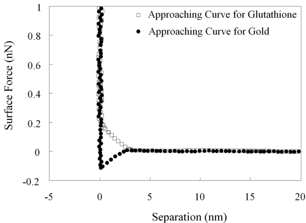
Fig. 2. Force-distance curve between a silicon nitride probe and the glutathione layer formed on the gold surface in 100 mM potassium nitride at pH 8.
