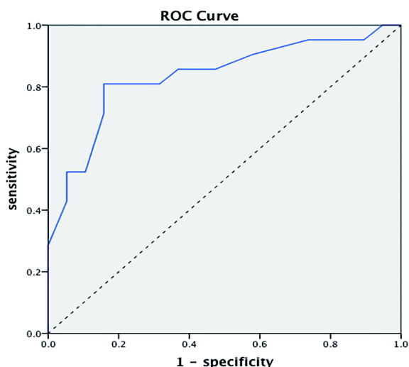
Figure 4. Dukes C-D Stage was Distinguished from A-B stage by MiR155. In Receiver Operating Characteristics (ROC) curve analysis, when C-D stage was differentiated from A-B stage by miR155 with an AUC of 0.835 (95% CI: 0.706-0.963), the best cutoff value was 0.125 with 81.0% sensitivity and 84.2% specificity
