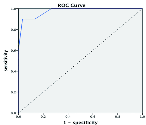
Figure 3. N2 Stage was Distinguished from N0-1 Stage by MiR155. In Receiver Operating Characteristics (ROC) curve analysis, when N2 stage was differentiated from N0-1 stage by miR155 with an AUC of 0.975 (95% CI: 0.930-1.000), the best cutoff value was 0.165 with 90% sensitivity and 96.7% specificity
