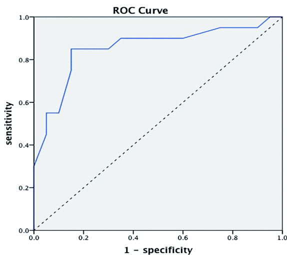
Figure 2. N1-2 Stage was Distinguished from N0 Stage by MiR155. In Receiver Operating Characteristics (ROC) curve analysis, when N0 stage was differentiated from N1-2 stage by miR155 with an AUC of 0.855 (95% CI: 0.730-0.980), the best cutoff value was 0.125 with 85.0% sensitivity and 85.0% specificity
