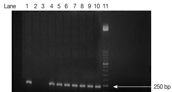
Fig. 1. Agarose gel electrophoresis analysis of SAG2 PCR amplification products. Second amplification of the 5' end of SAG2 locus. Lane 1, positive control. Lanes 2, 3, negative controls. Lanes 4-10, some positive samples (241 bp). Lane 11, 50-bp DNA marker.
