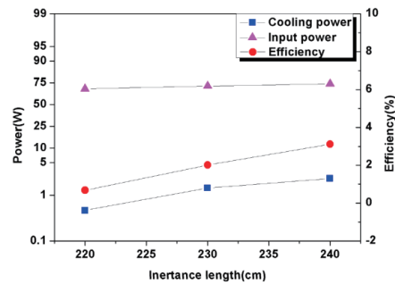
Fig. 7. Effect of inertance length on cooling power, input power, and efficiency
