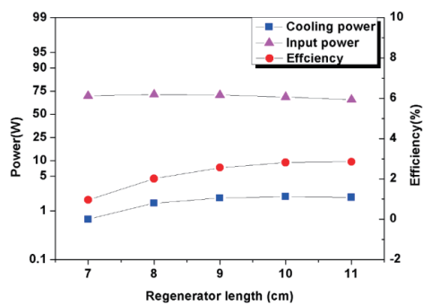
Fig. 9. Effect of regenerator length on cooling power, input power, and efficiency
