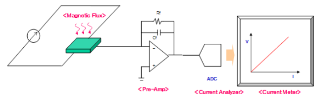
Fig. 6. Hall element current sensor measuring system using Ni-Fe core.
