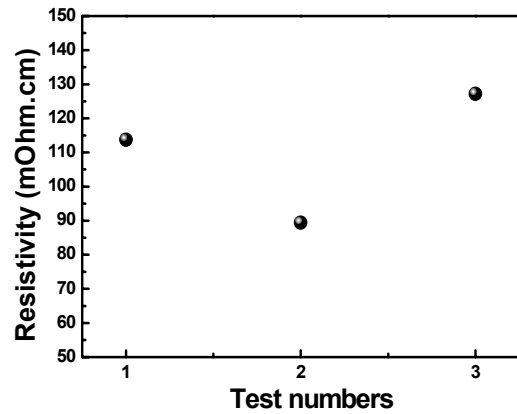
Fig. 5. Resistivity of fabricated Ni-Fe core samples.
