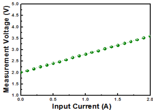
Fig. 8. Current-voltage system of Hall element current sensor measuring system using Ni-Fe core.
