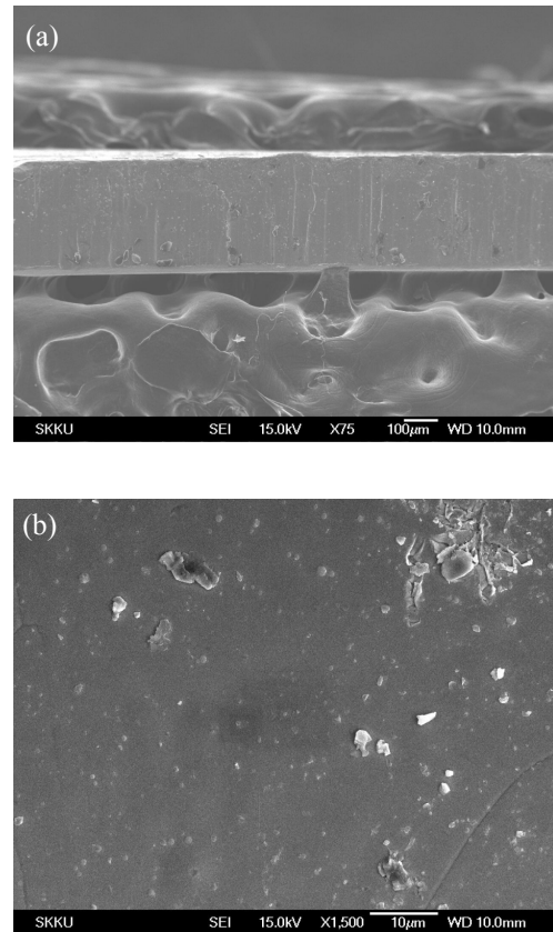
Fig. 1. (a) Cross-sectional and (b) surface images of fabricated Ni-Fe (Nickel steel) sample.
