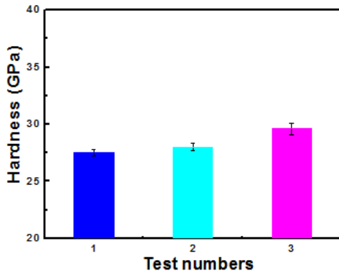
Fig. 3. Hardness values of fabricated Ni-Fe samples.
