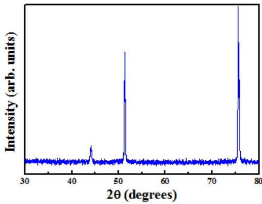
Fig. 2. XRD patterns of fabricated Ni-Fe sample.
