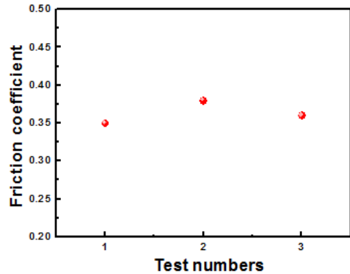
Fig. 4. Friction coefficient values of fabricated Ni-Fe core samples.
