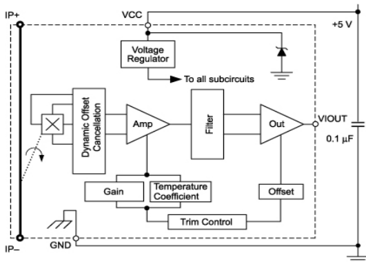
Fig. 7. Block diagram of Hall element current sensor measuring system using Ni-Fe core.
