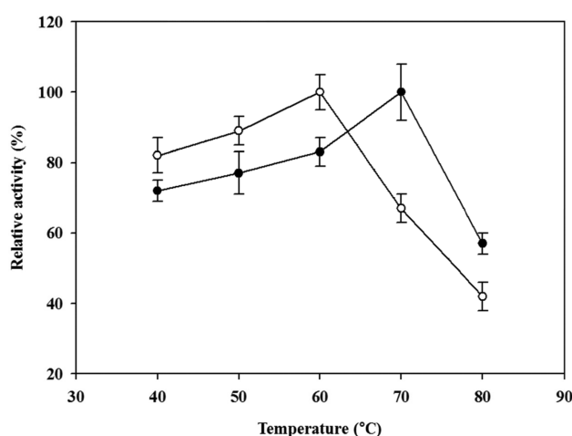
Fig. 2. Effect of temperature on endo- \beta -1,4-glucanase (●) and endo- \beta -1,4-xylanase (○) activities by Thermoascus aurantiacus .
