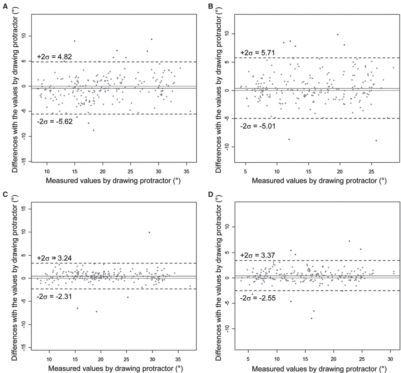
Fig. 5. Bland-Altman plots. (A) The distribution of the bucco-lingual convergence angle differences between the measurements by CAD and drawing protractor, (B) The distribution of the mesio-distal convergence angle differences between the measurements by CAD and drawing protractor, (C) The distribution of the bucco-lingual convergence angle differences between the measurements by digital protractor and drawing protractor, and (D) The distribution of the mesio-distal convergence angle differences between the measurements by digital protractor and drawing protractor are shown. The solid lines represent the mean values of the differences between the two methods. The dashed lines are \pm 2s of the measured value differences between two methods. s ; standard deviation.
