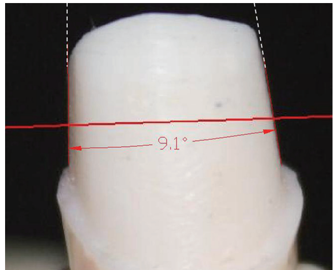
Fig. 4. The measurement of the abutment occlusal convergence angle by CAD. The two tangent lines (red solid lines) are mesio-distally established to the cervical third of the abutment. The software virtually extends the tangent lines to converge (white dashed lines) and calculates the angle between the tangent lines. Therefore, additional space, which the tracing method requires, is unnecessary.
