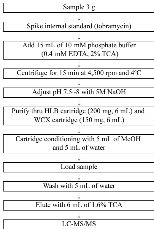
Fig. 2. Analytical procedure of aminoglycosides in meat.
