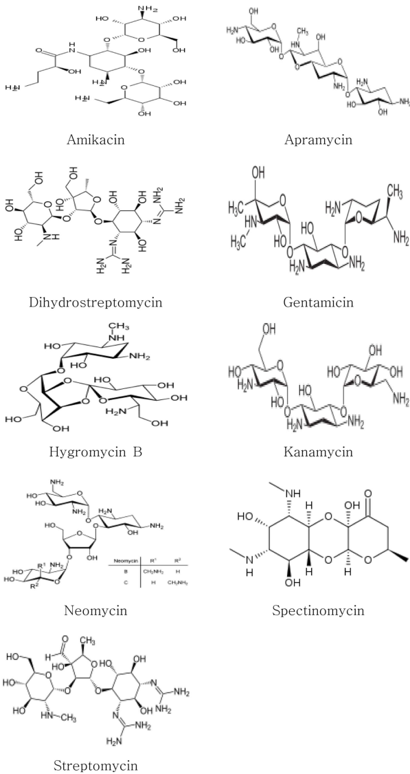
Fig. 1. Molecular structures of aminoglycosides.
