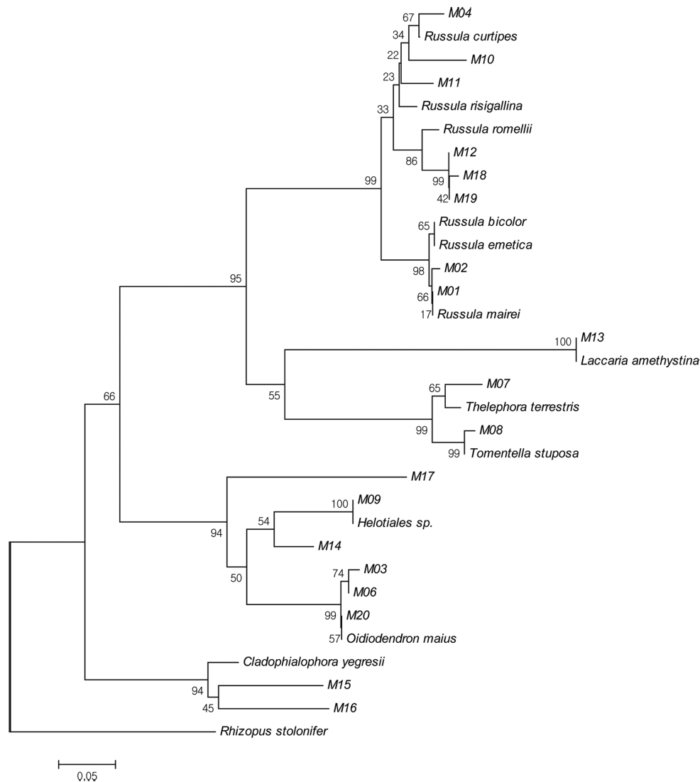
Fig. 1. Neighbour-joining tree of ITS rDNA sequences from ectomycorrhizal morphotypes and reference sequences obtained from GenBank. Rhizopus stolonifer was used as an outgroup and numbers at nodes indicate percent bootstrap support (1000 replicates).
