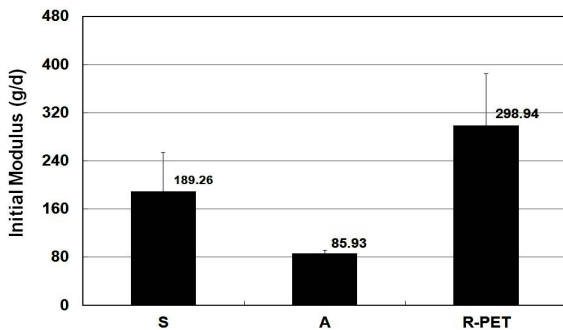
Figure 3. Initial modulus of coolness yarn specimens.
