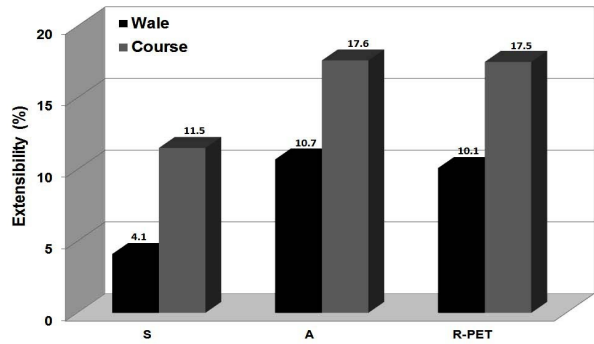
Figure 10. Extensibility of coolness knitted fabrics.
