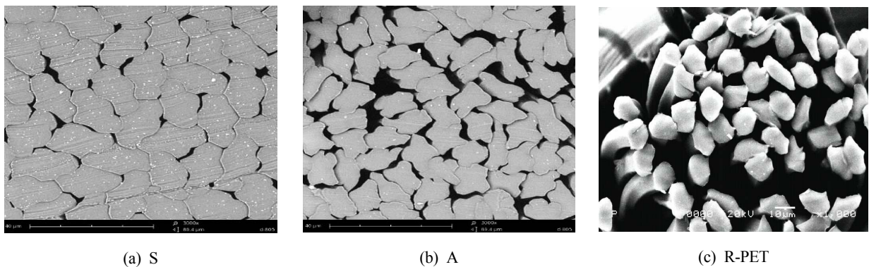
Figure 1. SEM photograph of cross-section of 3 kinds of yarn specimens.
