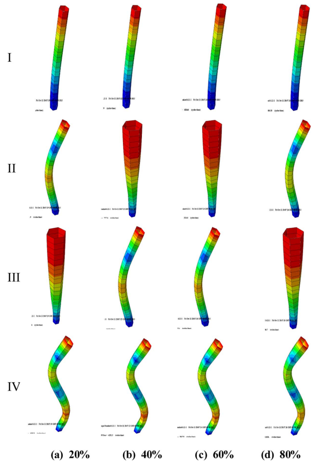
Fig. 5. Mode shapes for different fiber-volume fractions ( [0/90]_{4S} )
