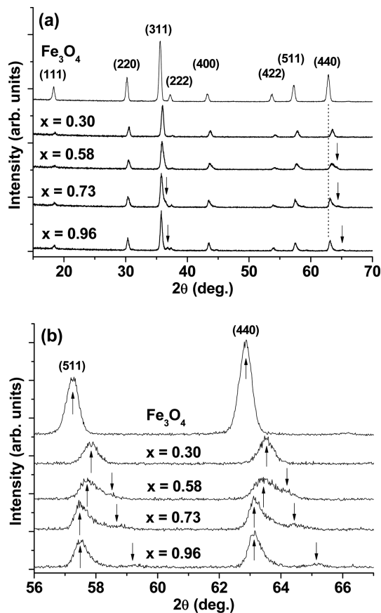
Fig. 1. (a) XRD patterns of polycrystalline \text{Ni}_x\text{Fe}_{3-x}\text{O}_4 thin films, and (b) Magnified (511) and (440) peaks of the XRD patterns.
