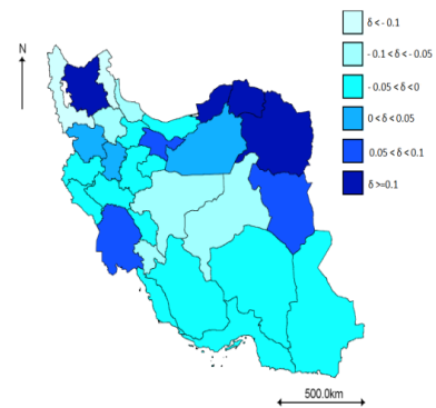
Figure 2. Post-Estimate values of \delta_i
