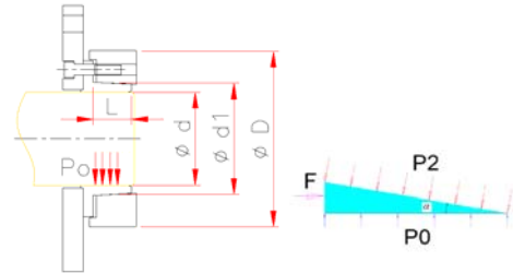
Figure 10: Assembly method and force diagram
