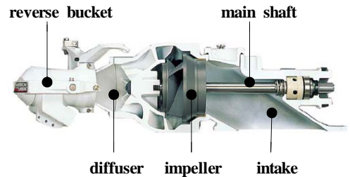
Figure 2: Inner shape of water jet
