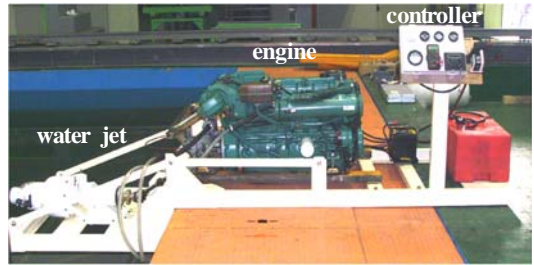
Figure 10: Installation of test bed on water tank
