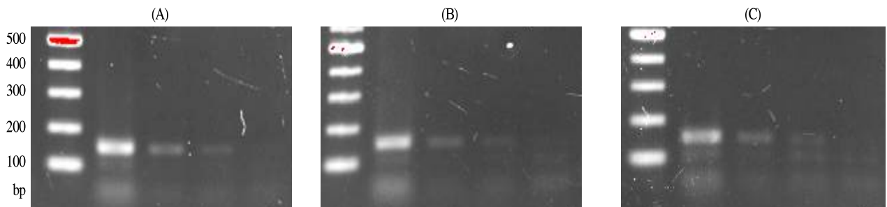
Fig. 2. Comparison of the two methods for concentrating HAV by RT-PCR assay. (A) The limit of detection for the RT-PCR assay was assessed with 10-fold serial dilutions of HAV stock.
