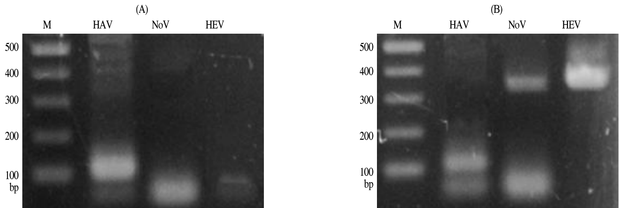
Fig. 1. RT-PCR assay for detecting enteric virus including hepatitis A virus (HAV), norovirus (NoV), and hepatitis E virus (HEV) using immunomagnetic separation (IMS).
